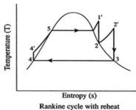
T-s diagram for steam
