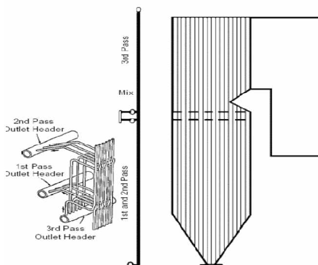
Figure 27: Multiple pass furnace design
