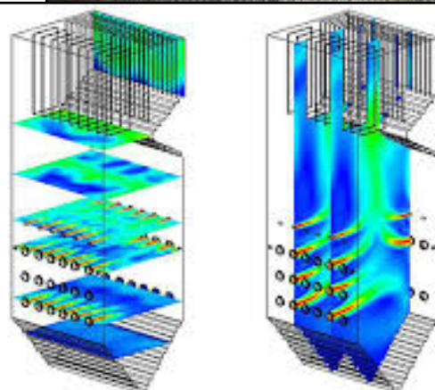
CFD velocity results, for opposed-fired furnace with OFA, showing good horizontal mixing and penetration.
